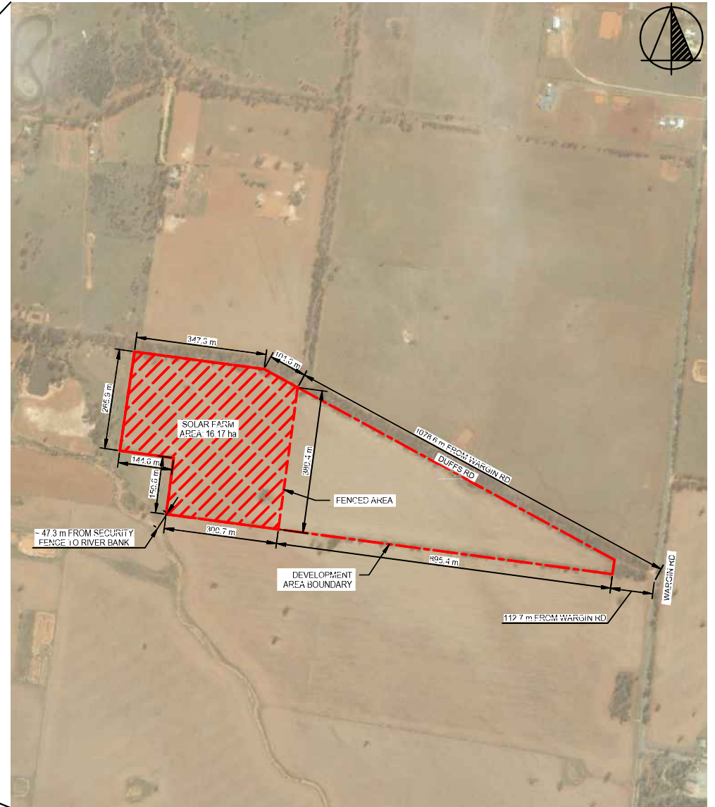
3 SITE PLAN SCALE: 1:10,000
